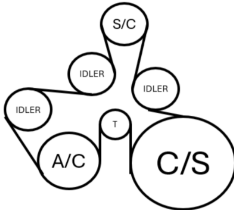
SUPERCHARGER BELT ROUTING DIAGRAM
