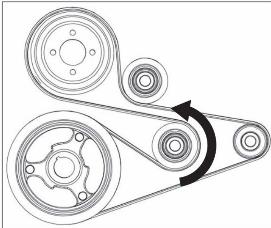
FACTORY FEAD BELT ROUTING DIAGRAM
